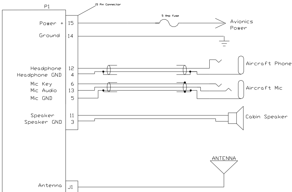
Figure 6: COM 2000 Basic Wiring Diagram
